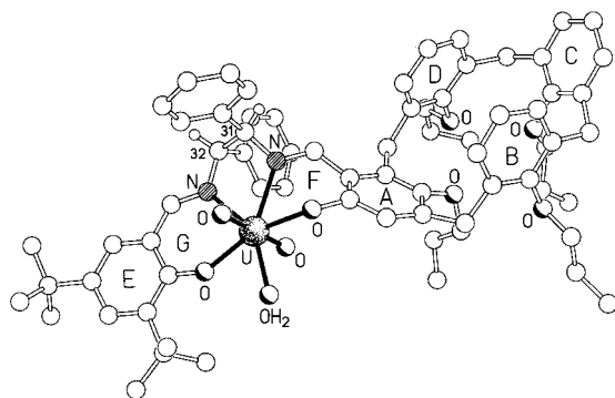
Figure 2. The molecular structure of 9 .
