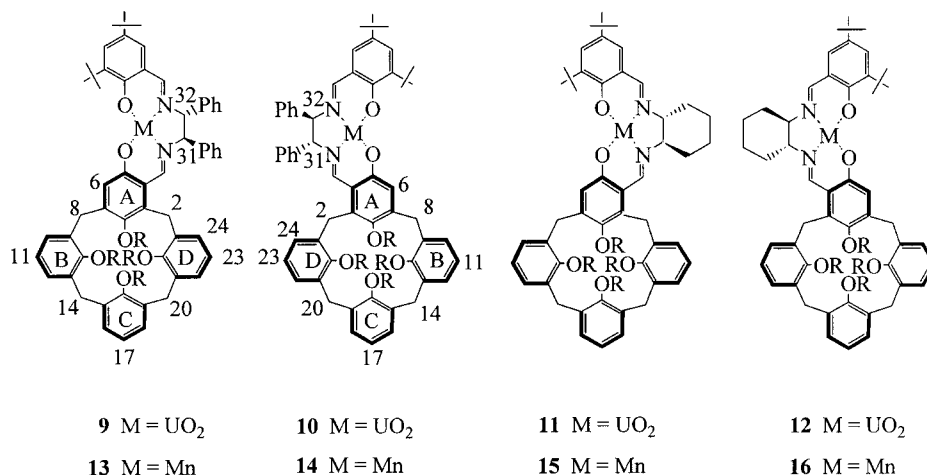
Scheme 2. Mn III and UO 2 salen calix[4]arene complexes.
