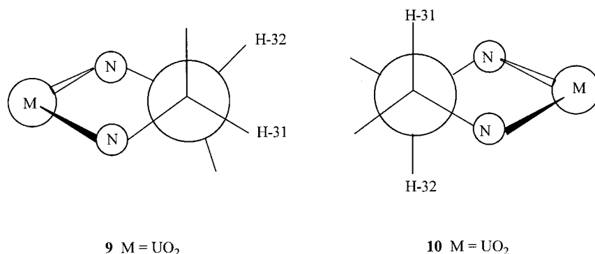
Figure 1. Newman projection of the diimine bridge.
