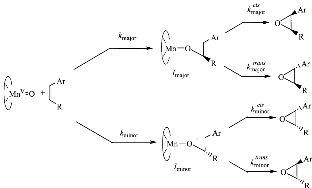
Scheme 3. Jacobsen nonstereospecific mechanism of alkene asymmetric epoxidation.
