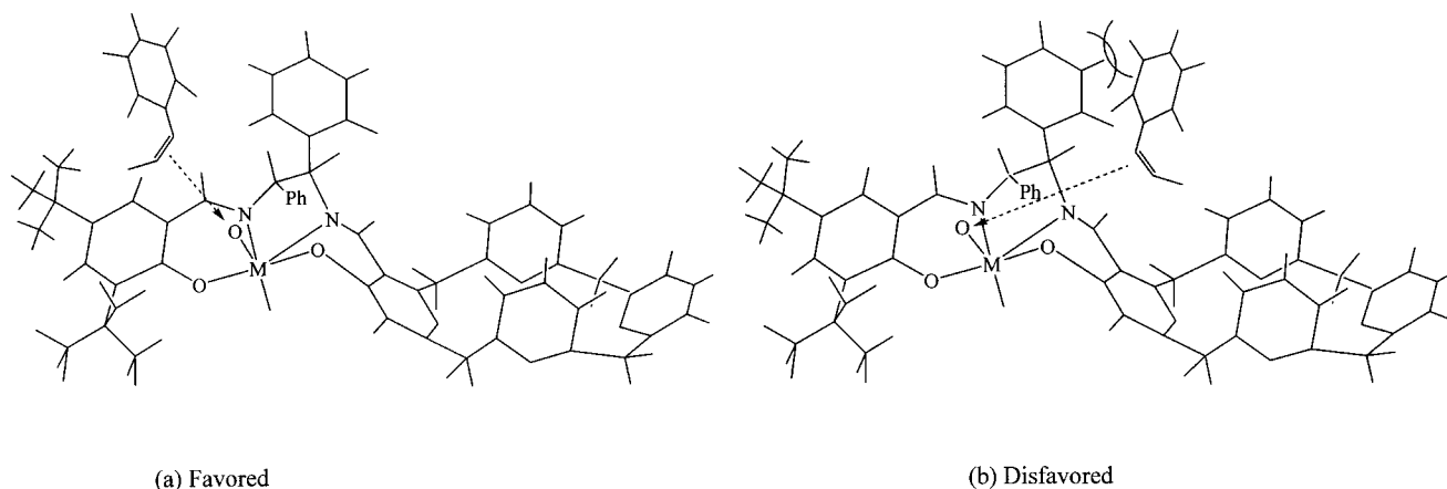
Figure 4. Approach directions for the epoxidation of cis - \beta -methylstyrene with catalyst 13 .
