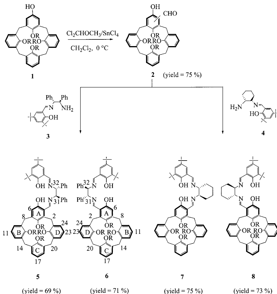
Scheme 1. Synthesis of salen ligands containing a calix[4]arene unit.
