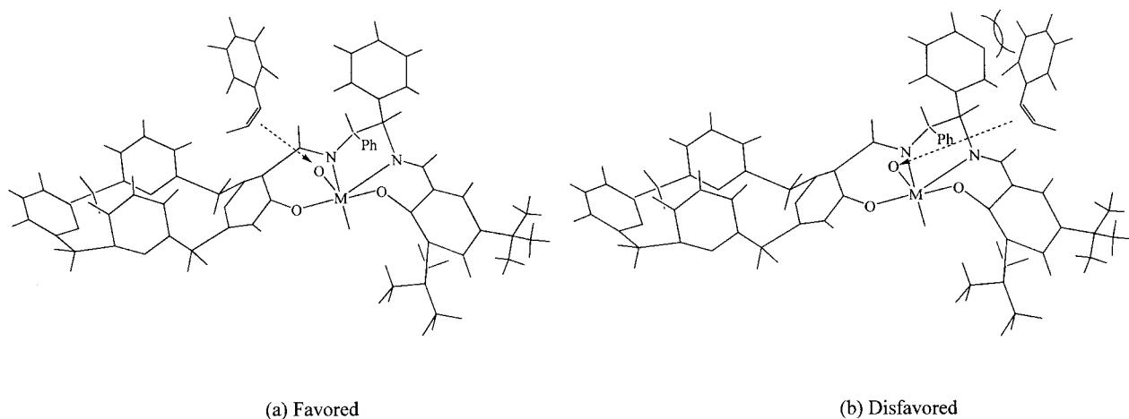
Figure 3. Approach directions for the epoxidation of cis -β-methylstyrene with catalyst 14 .
